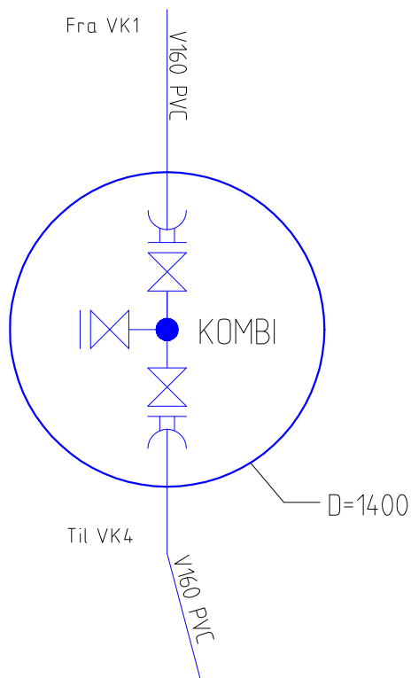
VK3 (DN1400 betong)
